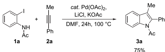
Scheme 1. Larock's direct annulation with unsymmetrical internal alkyne 2a .
