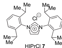
Figure 2. Imidazolium salt 7 .
