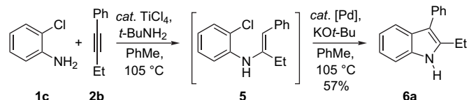
Scheme 4. One-pot synthesis of indole 6a used for the optimization of palladium catalysts.
