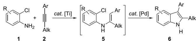
Scheme 3. Regioselective annulation of internal alkynes 2 .
