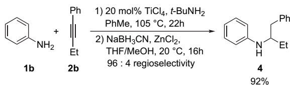
Scheme 2. \text{TiCl}_4 -catalyzed intermolecular hydroamination of alkyne 2b with formal anti-Markovnikov selectivity.
