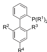
Figure 3. General structure of monophosphine biaryl ligands.
